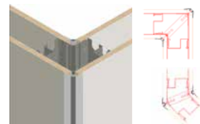
90° & 135° integrating discreet profiles
