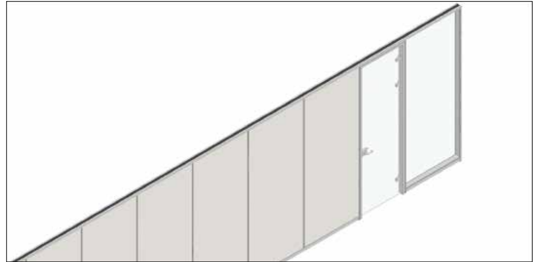
PARTITION WITH 12-14 MM PANELS VERSUS PARTITION WITH 18 MM PANEL.
