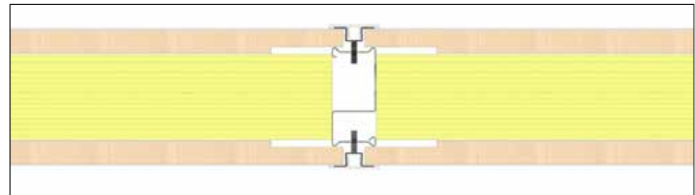
PARTITION WITH 12-14 MM PANELS VERSUS PARTITION WITH 18 MM PANEL.
